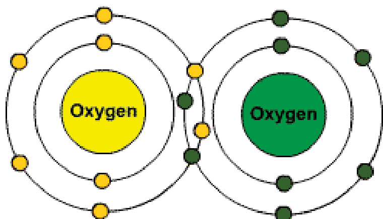
Oxygen molecule covalent bond
