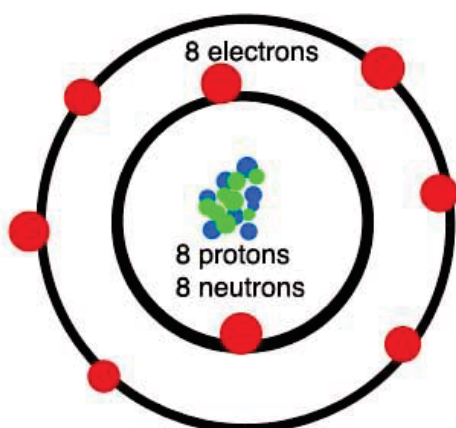
Oxygen atom
